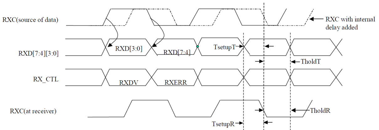
Figure 5-14 RGMII Interface Receive Timing
