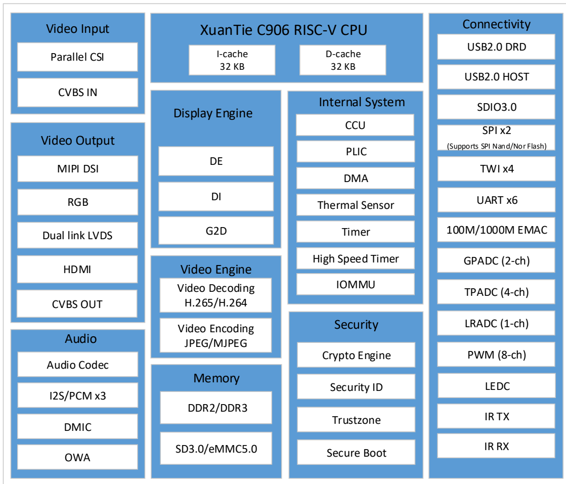
Figure 3-1 F133 MX-HXX System Block Diagram
