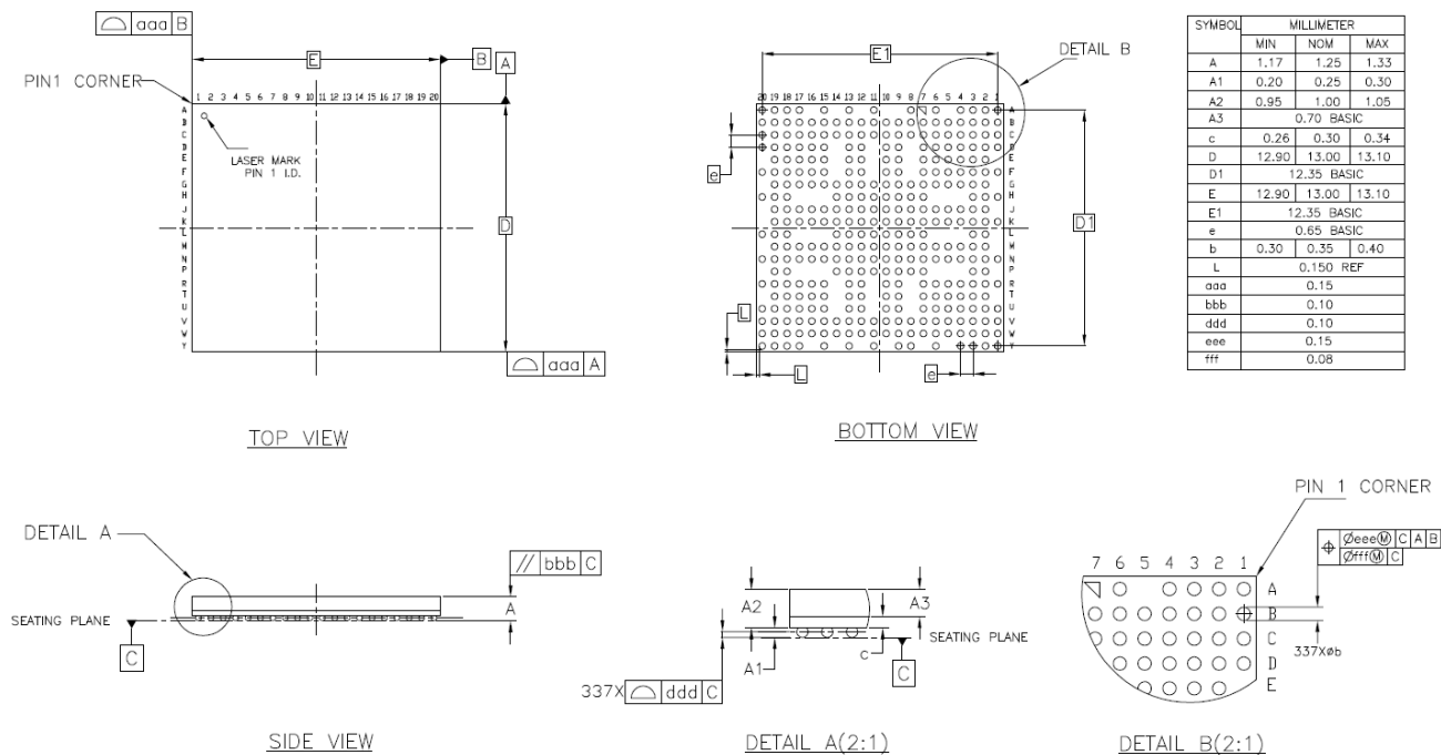
Figure 7-2 F133 MX-HXX Package Dimension
