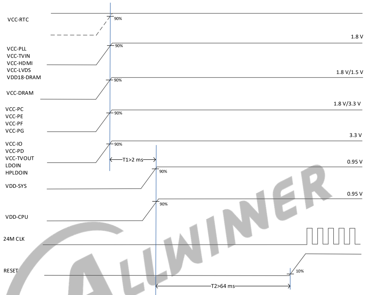
Figure 5-28 Power-On Timing
