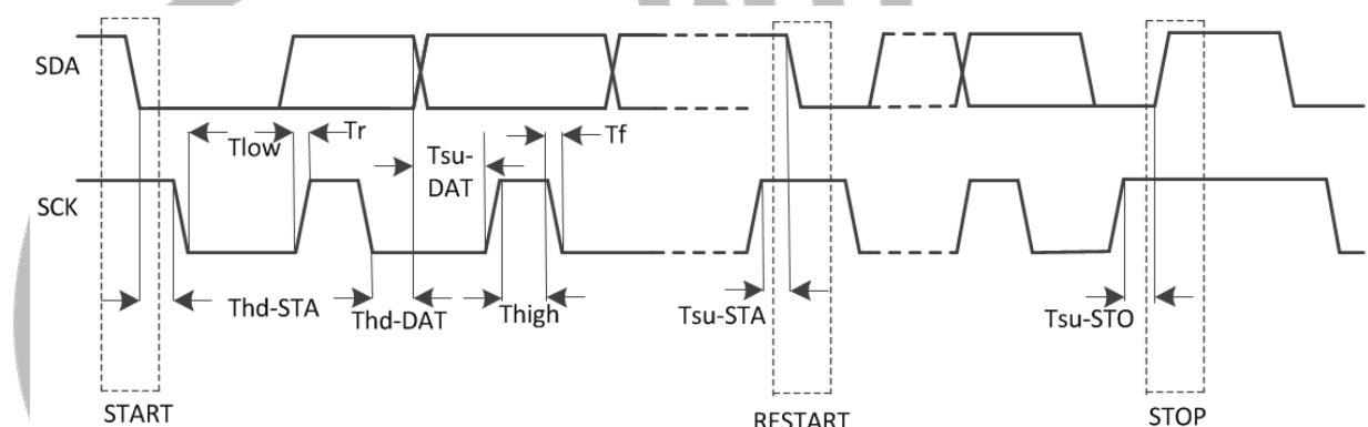
Figure 5-22 TWI Timing
