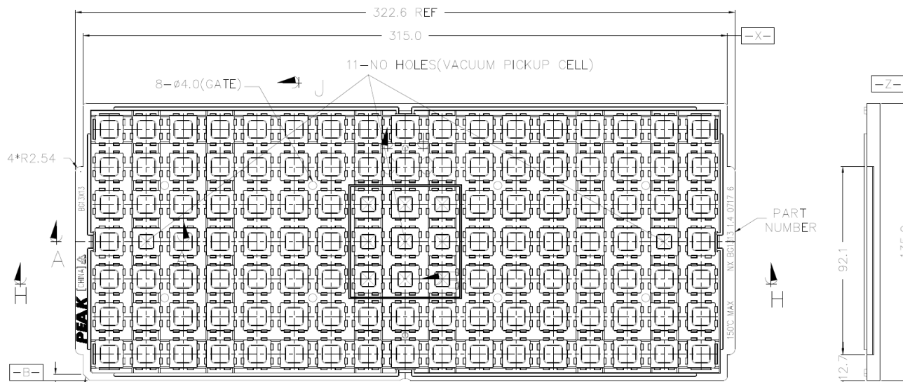
Figure 8-1 F133 MX-HXX Tray Dimension Drawing
