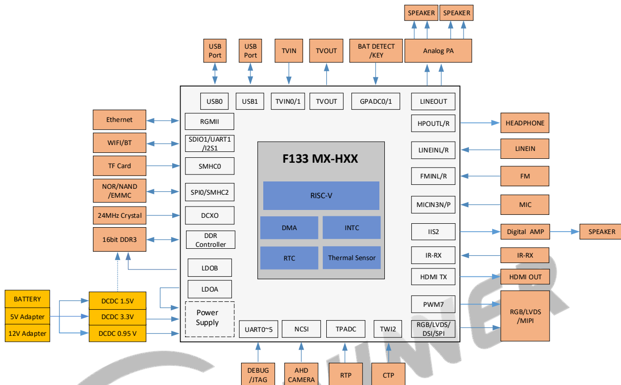
Figure 3-2 F133 MX-HXX Multi-Media Decoding Platform Solution
