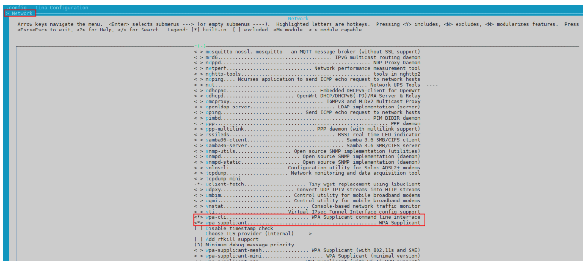
图 3-31: Tina-wpasupplicant 配置
