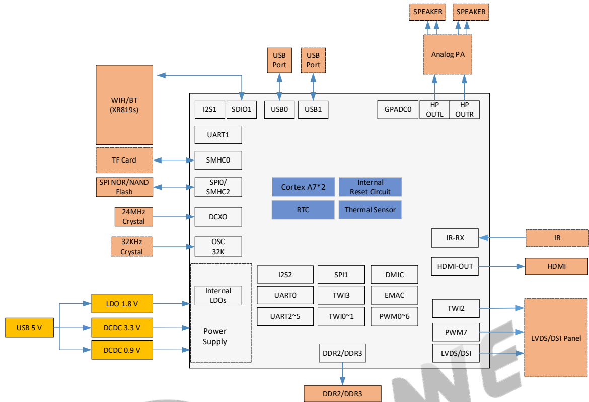
Figure 3-2 Intelligent Speaker with Screen Solution of the H133
