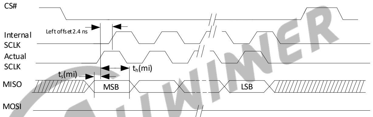
Figure 5-13 SPI Reading Timing
