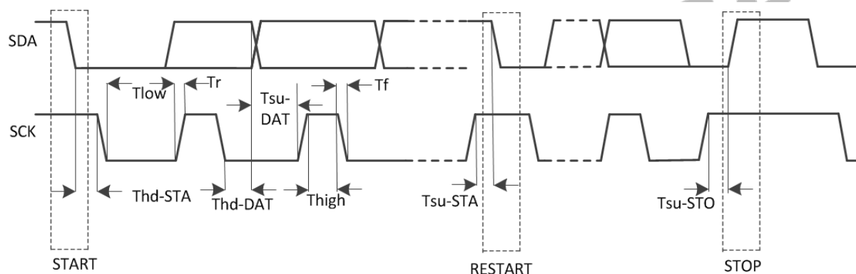
Figure 5-19 TWI Timing
