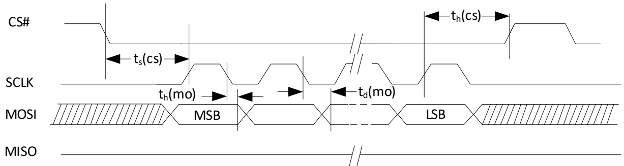
Figure 5-12 SPI Writing Timing
