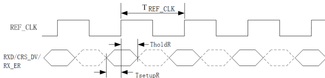
Figure 5-9 RMII Interface Receive Timing
