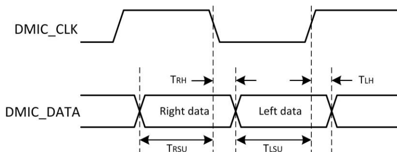
Figure 5-22 DMIC Timing
