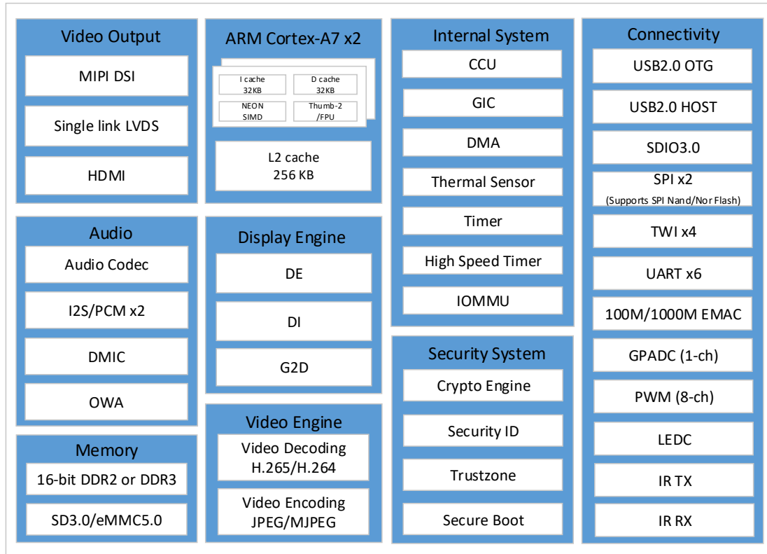
Figure 3-1 H133 System Block Diagram
