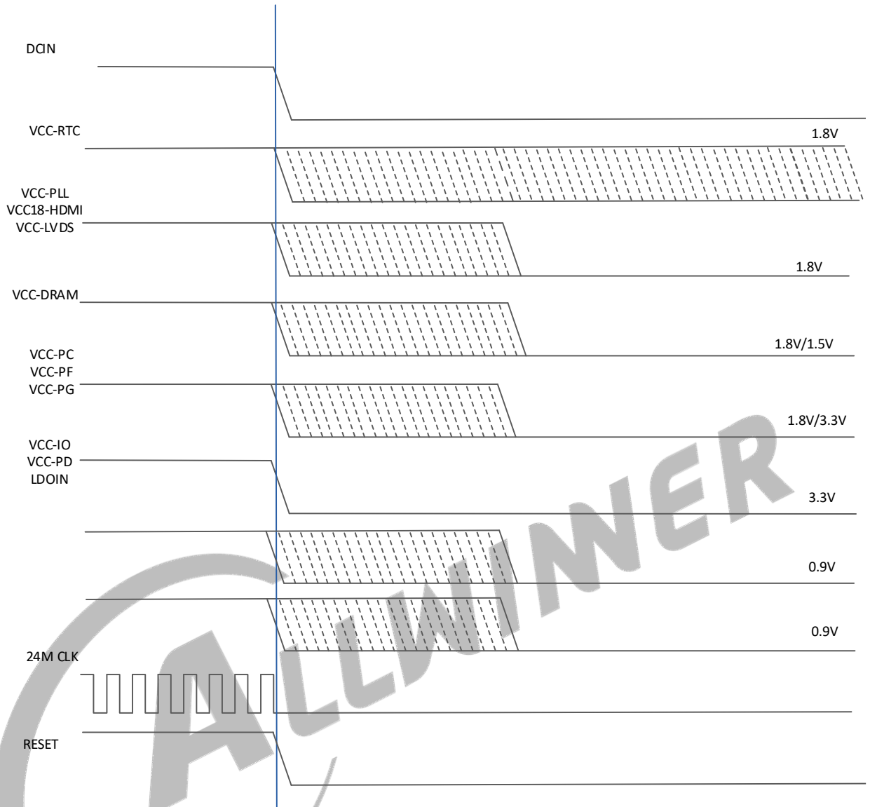
Figure 5-26 Power-Off Timing
