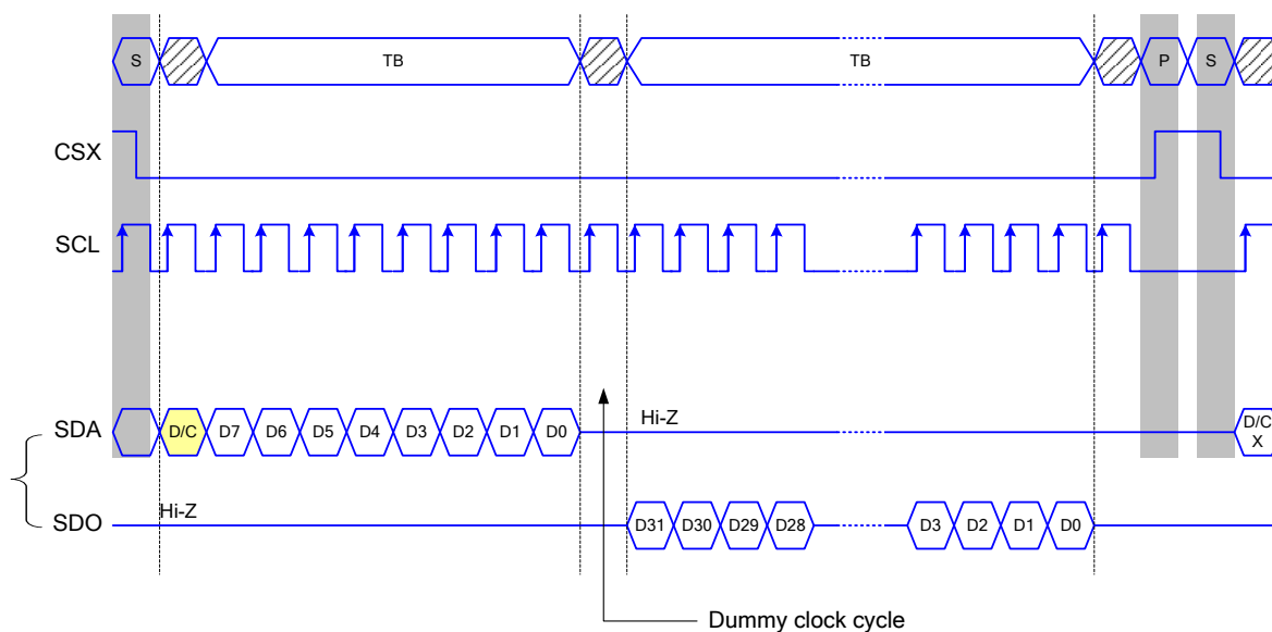
Figure 13 3-line serial interface read protocol
