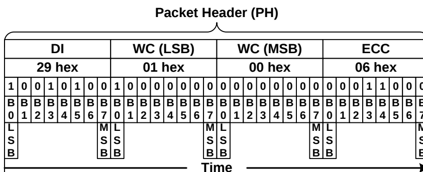
Figure 49 Packet Header (PH) on Long Packet (LP a )
